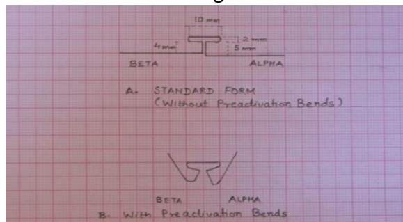
Fig.1 .017 X .025 TMA T loop spring for 6 mm activation with pre-activation bends
