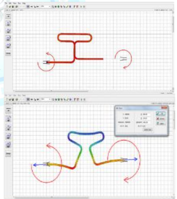
Fig. 3,4 .017 X .025 TMA T loop spring for 6 mm activation upon activation
